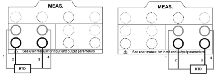
Figure 6 RTD measurement
