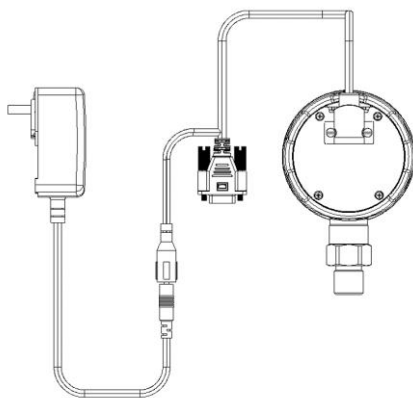
ADT680A/680P adapter diagram
