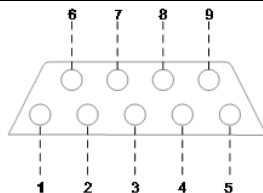
RS232 DB9 Female pins description diagram
