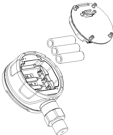
ADT680A/680P battery installation
