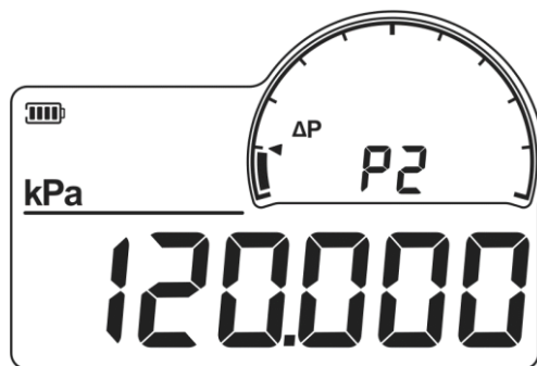
Figure 15 Leak test end pressure
