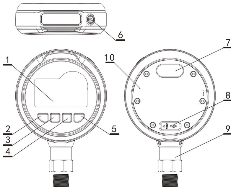
Figure 1 Basic Structure
